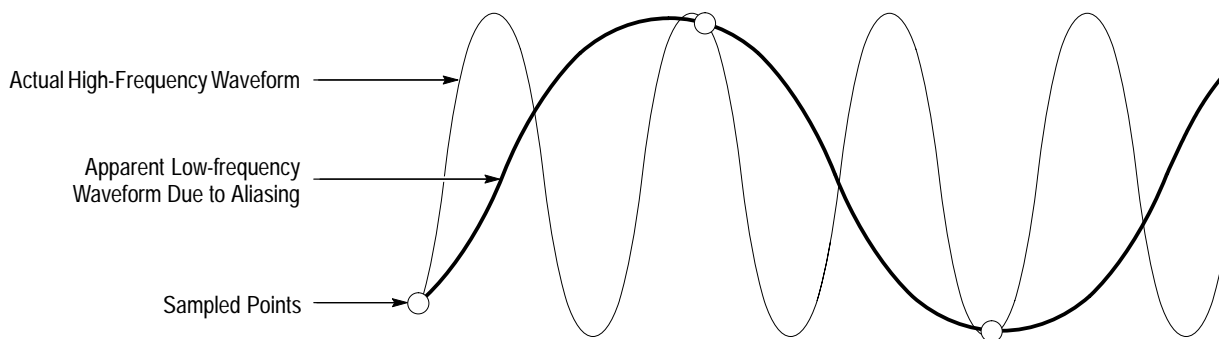
Figure 3–16: Aliasing
